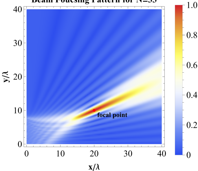
Beam Focusing Pattern for N=33
